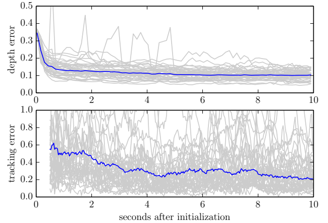
Figure 8: Initialization evaluation: development of errors in successful random initialization runs (average in blue, all samples in gray), evaluated on subsequences of the TUM RGB-D benchmark fr2/desk sequence. The depth error shows the relative deviation from the ground truth depth, after choosing the optimal scale. The tracking error shows the translational drift per 0.5 seconds, relative to the traveled distance. The largest reduction in depth error happens already within the first 0.5 seconds; the tracking error requires longer to stabilize.
