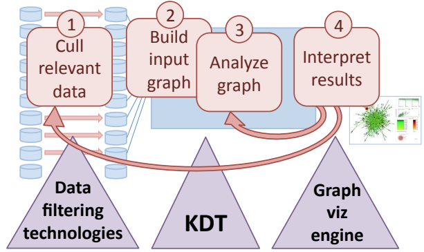
Figure 3: A notional iterative analytic workflow, in which KDT is used to build the graph and perform the complex analysis at steps 2 and 3.
