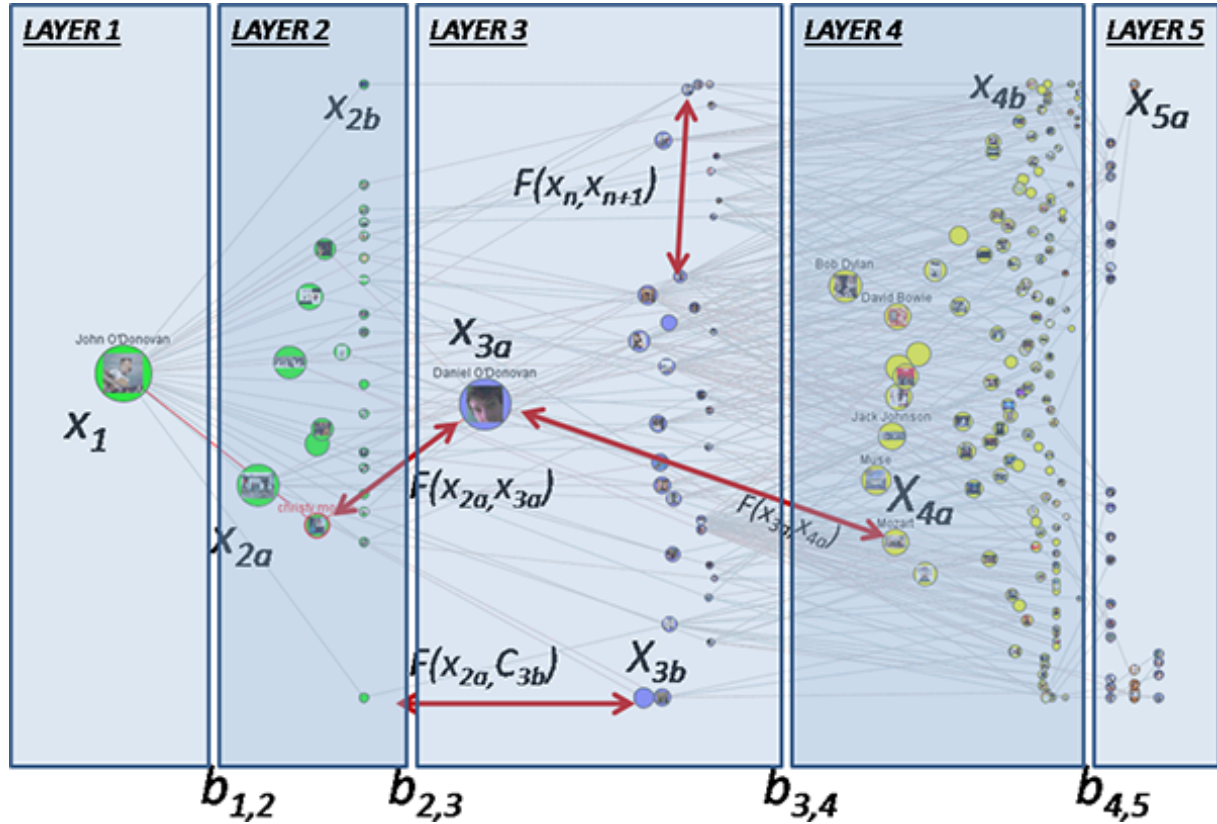
Figure 2: Description of various forces and constraints in the layout algorithm.
